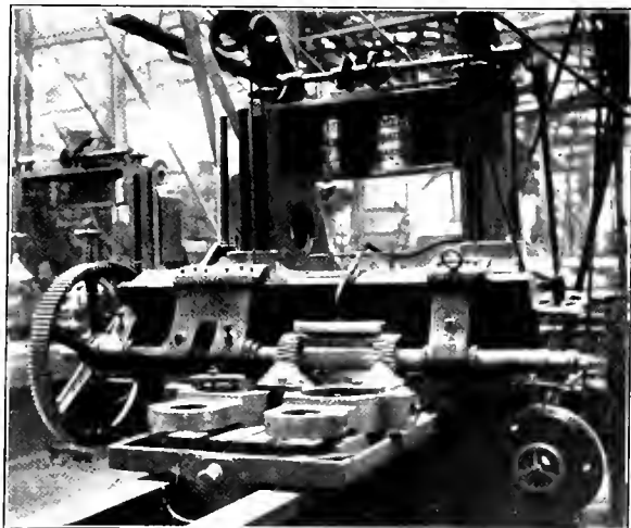
Fig. 9—Fluting the Main Rods
